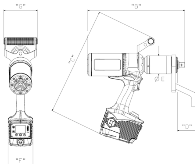
FIGURE 57 – Tool Dimensions
