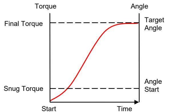
FIGURE 50 – Angle Mode
