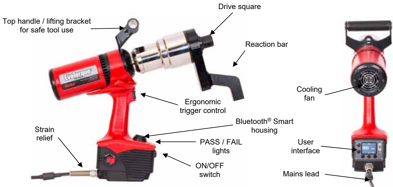
FIGURE 1 – Tool Features
