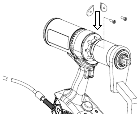
FIGURE 4 – Install infills
